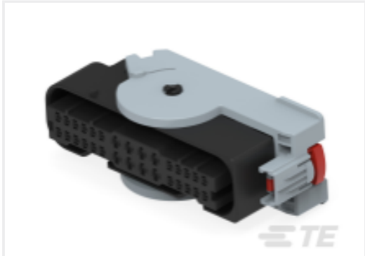
TE 产品编号5-2109446-2 MCP 1.5/2.8 SLD 30P PLUG ASSY
