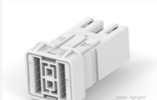
TE 产品编号2359563-1 2POS,HC-STAK 25,HDR INNER HSG ASSY,BXDU
