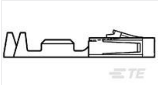
TE 产品编号1-104479-1 SHORT POINT RECP CONT LP
