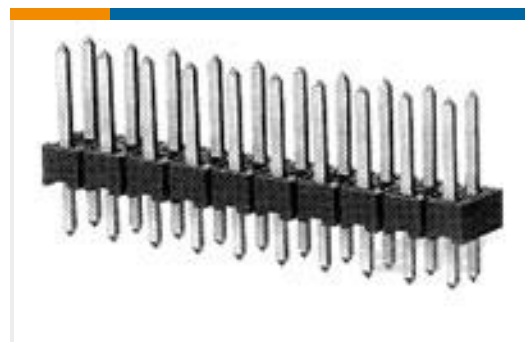
TE 产品编号5-146256-8 16 MODII HDR DRST B/A .100CL L
