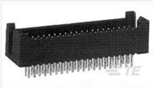
TE 产品编号6-534978-0 72 MODII 2PC HDR DR W/HLDWN, ROHS
