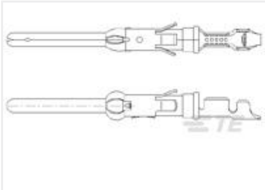
TE 产品编号163086-2 LOOSE PIECE PIN TYPEIII+ CONTACT SIZE 16
