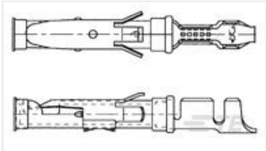
TE 产品编号1-163087-1 SPEC.PLATED
