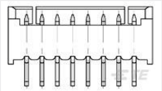
TE 产品编号4-1734598-2 1.25 WTB HDR DIP L3.7 2 POS
