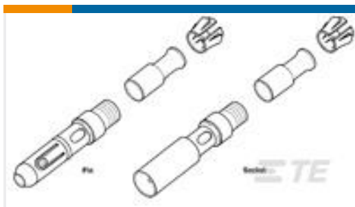
TE 产品编号9-328666-3 FERRULE, STEP DOWN, PLTD
