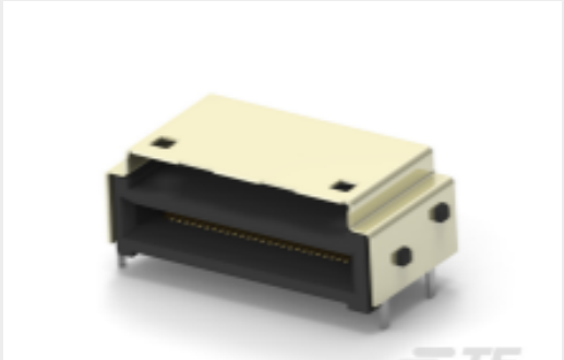
TE 产品编号2332208-3 RECEPT ASSY, RA, 56 POS, SLIVER 2.0
