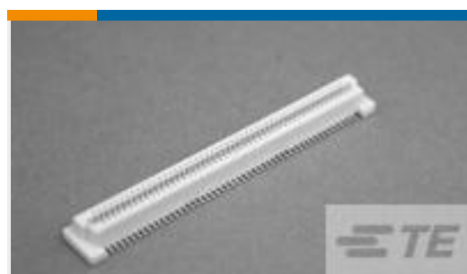
TE 产品编号5353999-5 0.8FH,R05H.5,120,30/Sn,TR,SC
