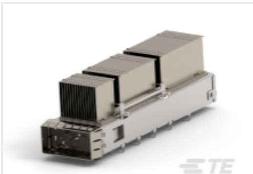
TE 产品编号2342934-3 QSFP-DD 1X1, STANDARD, W/ ZIPPER HS
