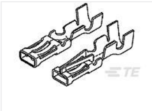
TE 产品编号770642-1 TIMER CONNECTOR TERMINAL 20-14 AWG PTPBR
