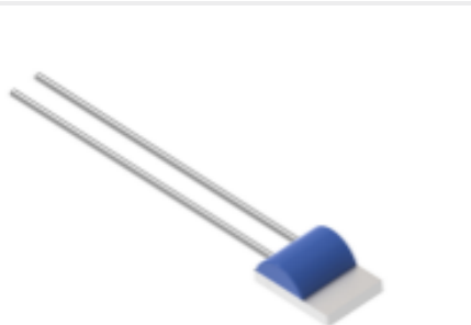
TE 产品编号NB-PTCO-159 Pt100, 2.0x2.3, Class C, PTFC101C1A0
