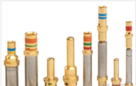
TE 产品编号38943-22L CONT SOC ASSY
