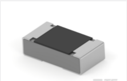
TE 产品编号9-2176480-4 RA73F 1J 5K11 0.1% 5K RL
