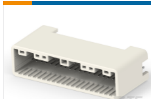
TE 产品编号2322794-1 40POS,TAB0.64X0.64,HDR ASSY, 180DEG,SLDR
