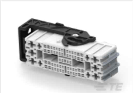
TE 产品编号2389766-1 66POS,HYBRID,REC HSG ASSY
