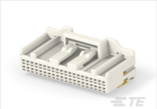
TE 产品编号2379277-1 40POS,TH 025,REC HSG ASSY,UNSLD, COD A
