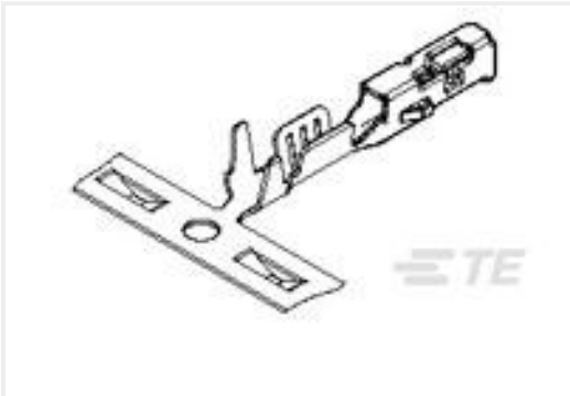
TE 产品编号2098165-1 CONTACT,FEMALE, 0.64, 20-22, C
