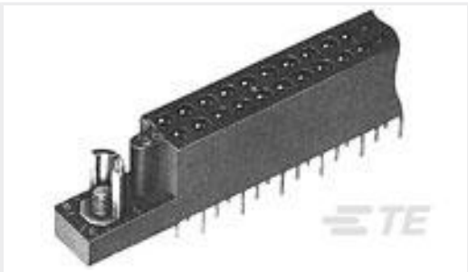
TE 产品编号531129-5 2 ROW BOX RECP 40 POS STAG
