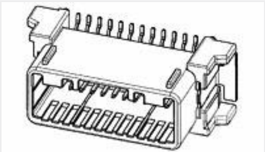
TE 产品编号1747642-2 0.64 SMD 40POS CAP ASSY V TIN
