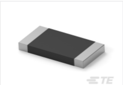
TE 产品编号3-2176421-8 TLRP 2512 2.0W R120 1% 25PPM 4K RL
