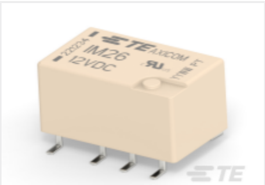
TE 产品编号3-1462039-1 IM26GR=IM RELAY 50mW 12V
