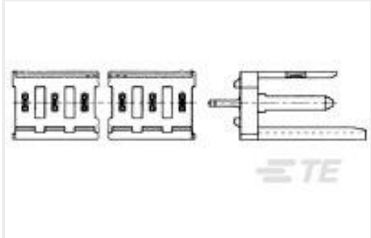
TE 产品编号280610-2 4P MOD 1 SHROUDED HEADER, ST, 0.4 Au
