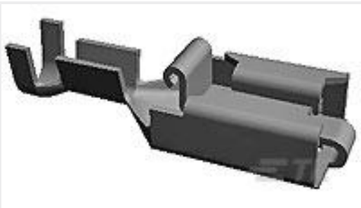
TE 产品编号927854-1 PL 250 REC TERMINAL 17-13 AWG BR
