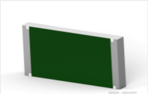
TE 产品编号2176405-6 3550 680R 5%
