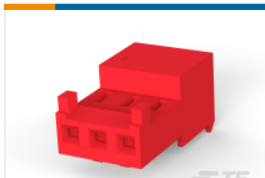
TE 产品编号3-644312-4 Nylon Tin Plated Receptacle: 2.54 mm, with Mating Alignment, MTA 100
