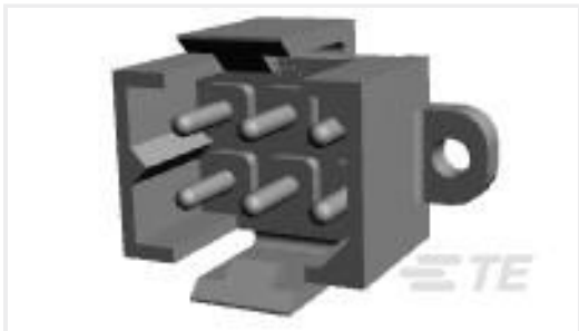
TE 产品编号1-207158-0 METRIMATE PIN HDR ASY,6P LF
