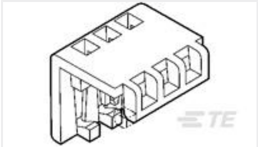
TE 产品编号643075-6 06P MTA100 MOLDED COVER
