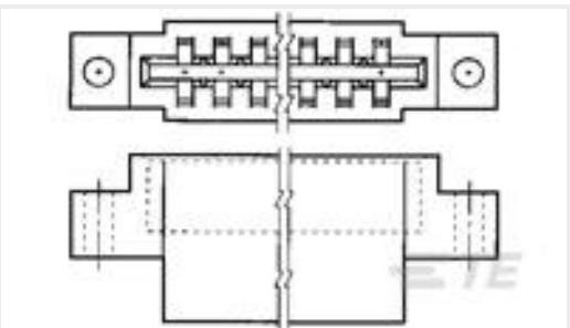
TE 产品编号583859-9 TW LF HSG 156 C/L
