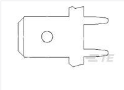
TE 产品编号1217539-1 250 FASTON,PCB TAB,TCBR
