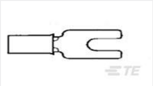
TE 产品编号40763 SPADE 138(3.50MM)TERMINAL 20-16 AWG TPBR
