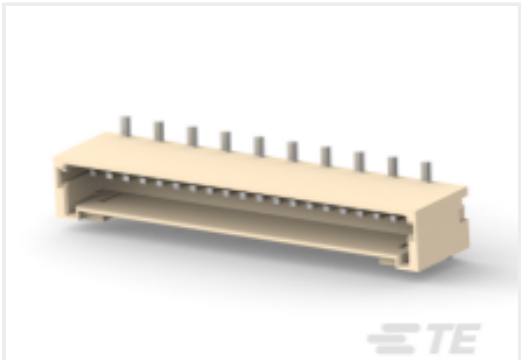
TE 产品编号 2-292371-0 SINGLE ROW POST HEADER ASS'Y SMT TYPE W/
