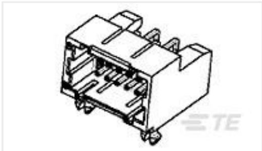
TE 产品编号 4-292262-0 DBL ROW (H) DIP TYPE WITH BOAR
