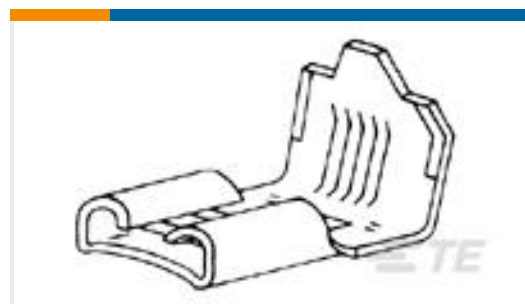
TE 产品编号62056-2 250 FASTON FLAG REC 18-12 AWG SPBZ
