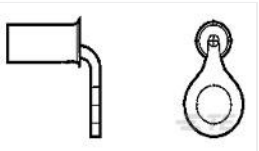
TE 产品编号321265 TERMINAL,SOLIS R 4/0 3/8 90DEG
