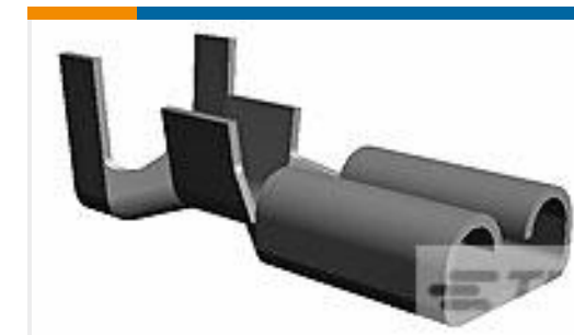
TE 产品编号62137-2 187 FASTON REC 20-16 TPBR
