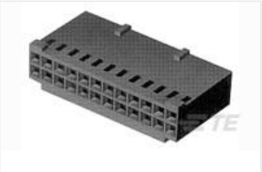
TE 产品编号2-87977-9 08 MODIV HSG COMP DR .100 POL
