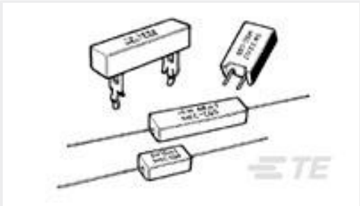
TE 产品编号2-1623795-7 SQP5 100R 5% WIRE
