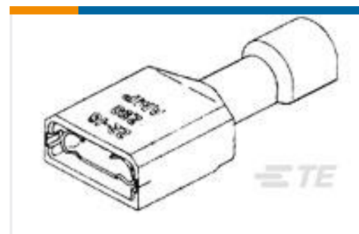
TE 产品编号4-520447-2 ULTRA-FAST 250 ASY REC 12-10 AWG TPBR
