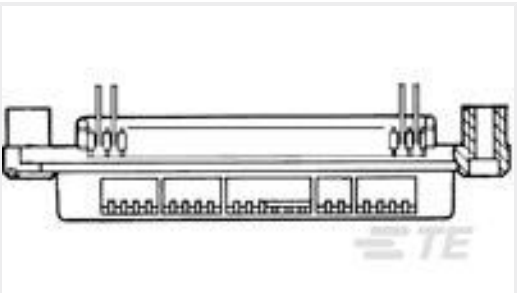
TE 产品编号5552246-1 ASSY, RCPT, 64 POS, VERT MTG
