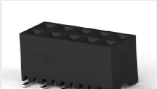
TE 产品编号1-2314844-0 10P,2MM,B-B,REC,DRV,T,SMD,0.1AU, TB,W/CP
