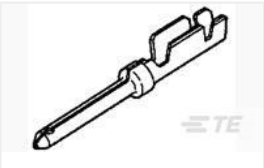
TE 产品编号1658670-2 PIN CONTACT,22-28 AWG, 22 DF, AMPLIMITE
