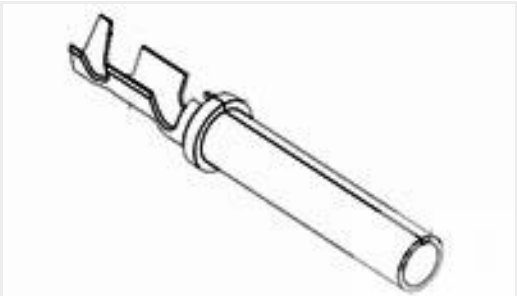
TE 产品编号776493-1 SOC, SF, SIZE 16, 18-20 AWG, AU/SN
