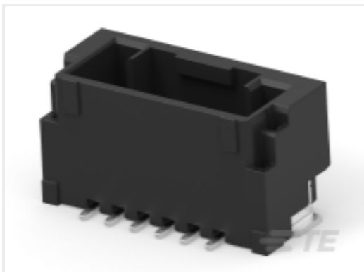
TE 产品编号2-2360540-6 SGI 1.25 HDR, 6P, VT, Key B, Black
