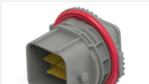
TE 产品编号2-2366509-2 48POS,HYBRID,PIN HSG ASSY,SLD, COD B
