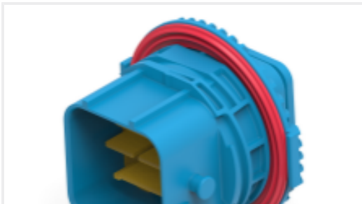
TE 产品编号2-2366509-4 48POS,HYBRID,PIN HSG ASSY,SLD, COD D
