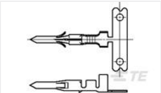
TE 产品编号770983-1 .062 COMM P&S PIN 18-24 PTPBR
