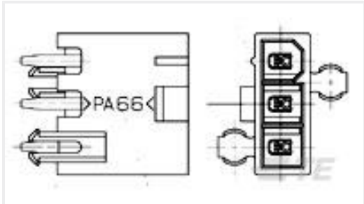
TE 产品编号2029181-3 3P VAL-U-LOK VRTHDR W/PGS GW
