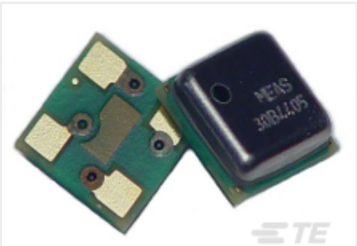
TE 产品编号MS563730BA03-50 30 BAR INDUSTRIAL ALTIMETER SENSOR
