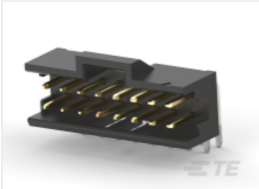
TE 产品编号 2-2823552-6 26P,2MM,PL HDR,DRRT,2.8,0.76AU,TR
