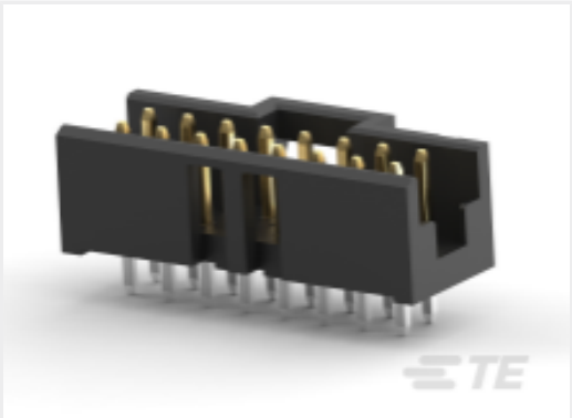
TE 产品编号 2-2823214-6 26P,2MM,PL HDR,DRVT,2.2,0.38AU,TB
