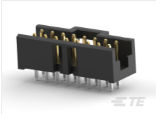
TE 产品编号 2-2823940-6 26P,2MM,PL HDR,DRVT,2.8,0.76AU,TB W/CAP
