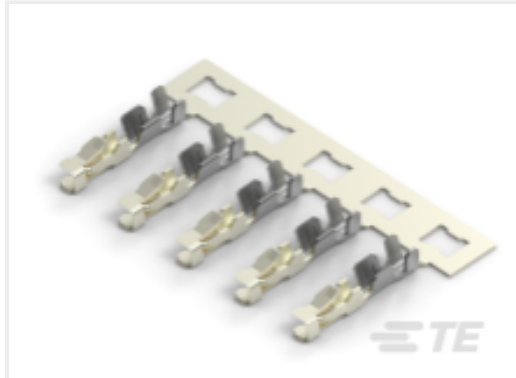
TE 产品编号 5-2316113-5 2MM,REC,CNT,CRIMP,24-28AWG,0.76 UM,APPL
