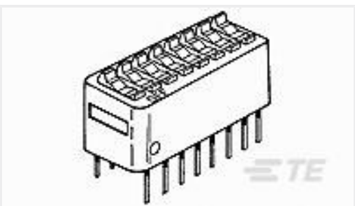
TE 产品编号3-435640-6 DIP SW 5 POSN SEALED
