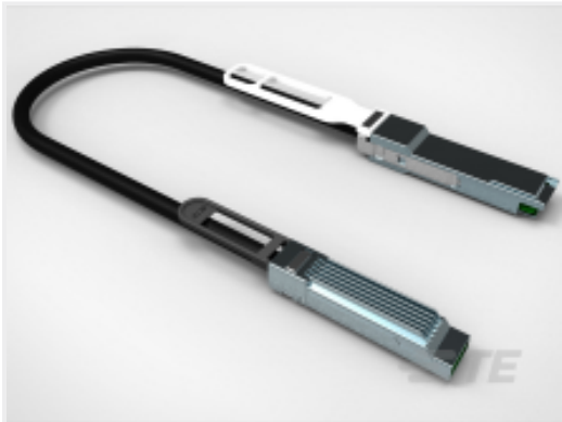
TE 产品编号 2821782-3 MICROQSFP TO QSFP28, 2M 28AWG
