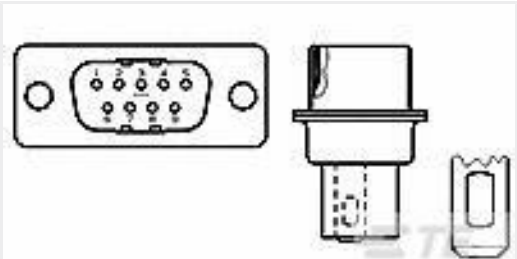
TE 产品编号215711-1 09P.HDP20 PLUG ASSY
